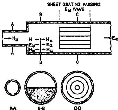
Baffle-plate converter inserted in a circular wave guide ahead of a coaxial sheet grating to convert H_{1,1} wave into E_{0,1} wave and vice versa. Cross sections are shown at the wave guide A-A, the baffle plate B-B, and the coaxial sheet grating C-C.
